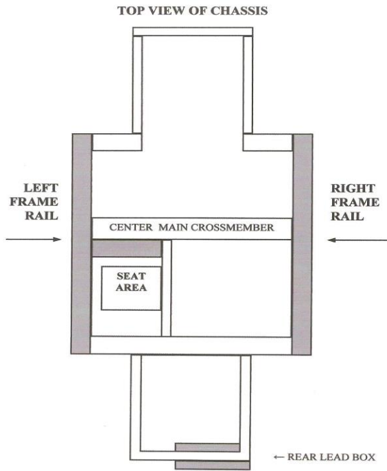
LEAD PLACEMENT ON FRAME
