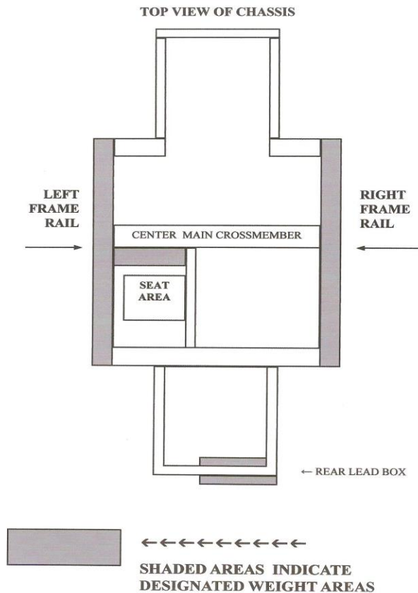
LEAD PLACEMENT ON FRAME
